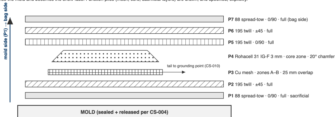
Figure 1: Figure 1. The §7.3 example stack drawn in section. P1 touches the mold and becomes the show face; function plies are drawn, and specified, explicitly.
